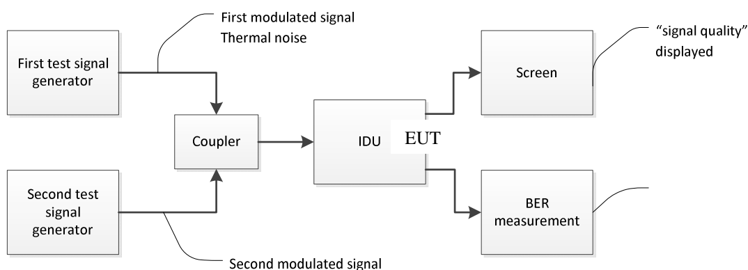
Figure 10: Test arrangement - adjacent signal selectivity
